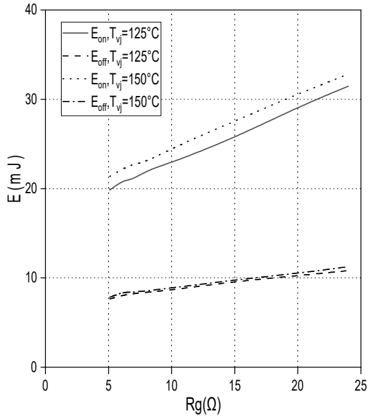
开关损耗 IGBT, 逆变器 (典型值) Switching losses IGBT, Inverter (typical) V_{GE} = \pm 15V, I_C = 150A, V_{CE} = 600V
